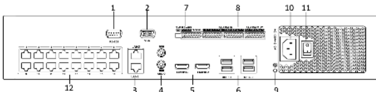
Figure 1-2 Rear Panel
